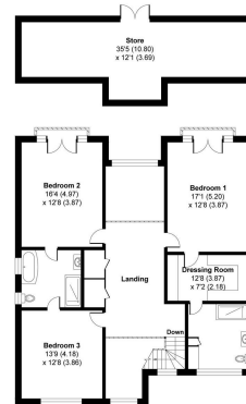
FIRST FLOOR
